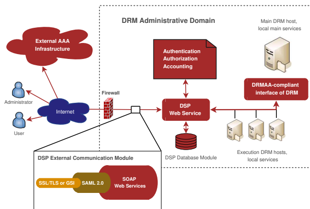
Figure 2. OpenDSP architecture
